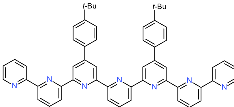
4'',4''''-Bis[4-(1,1- dimethylethyl)phenyl]- 2,2':6',2'':6'',2''':6''',2''''':6''''',2''''''- septipyridine
